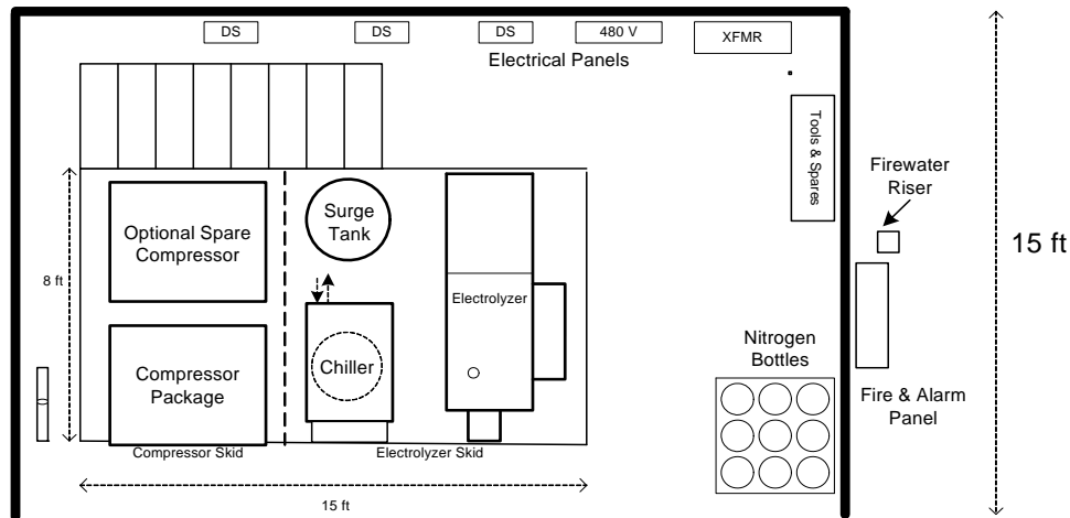
Plan View 1st Level
