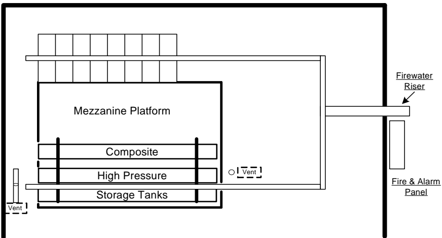
Plan View 2nd Level
